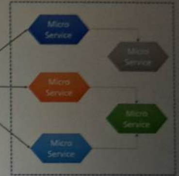
Kafka Streams
