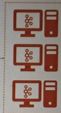
Kafka Broker
