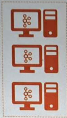
Kafka Broker
