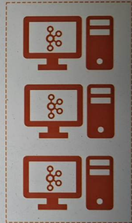
Kafka Broker
