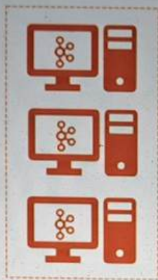
Kafka Broker
