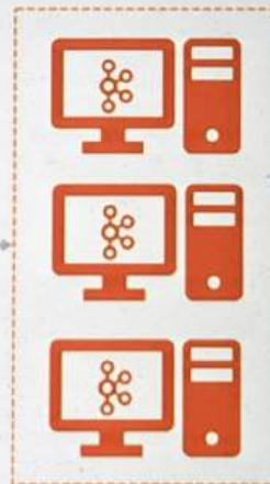
Kafka Broker
