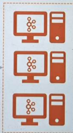
Kafka Broker
