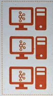
Kafka Broker
