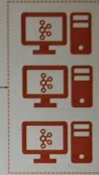
Kafka Broker
